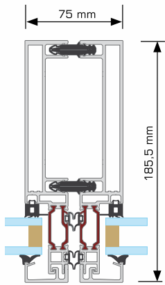
Mullion cross-section
