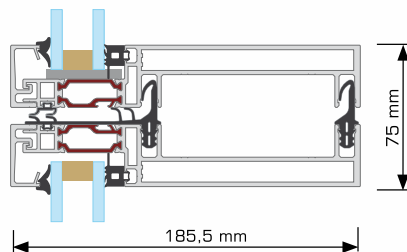
Transom cross-section
