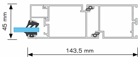
Door - cross-section
