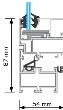
Opening window - cross-section
