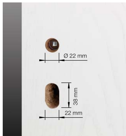
Door preparation for HOPPE handle sets on mini rose with escutcheons.
