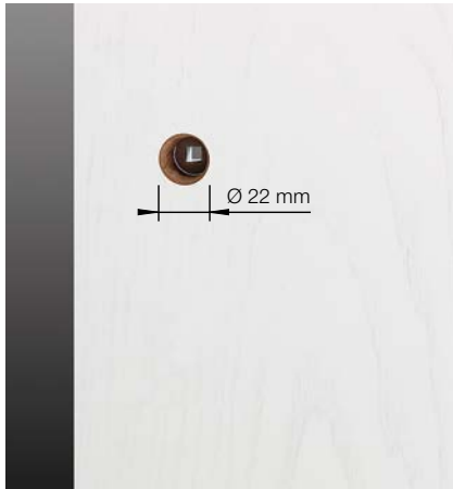
Door preparation for HOPPE handle sets on mini rose without escutcheons.
